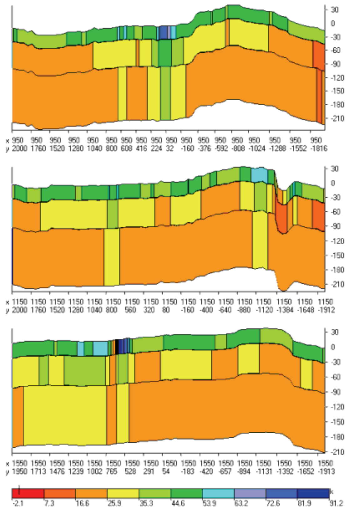
figure 10 – NW-SE sections along lines on 950, 1150, 1550 pickets.
