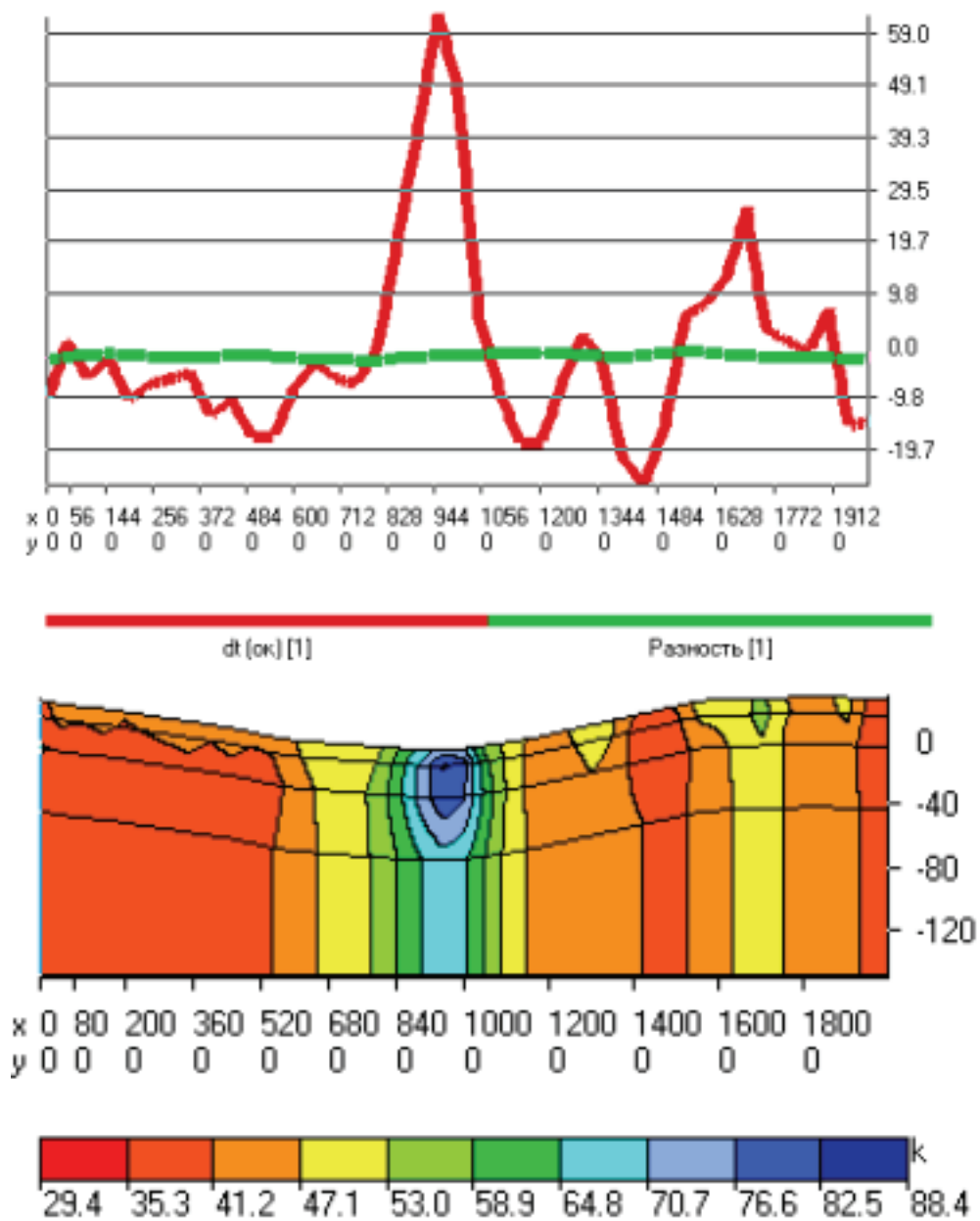
figure 14 – Plot of magnetic field along latitudinal profile 100 ( dt(ok) –initial and differential) and section obtained from one-level data.
